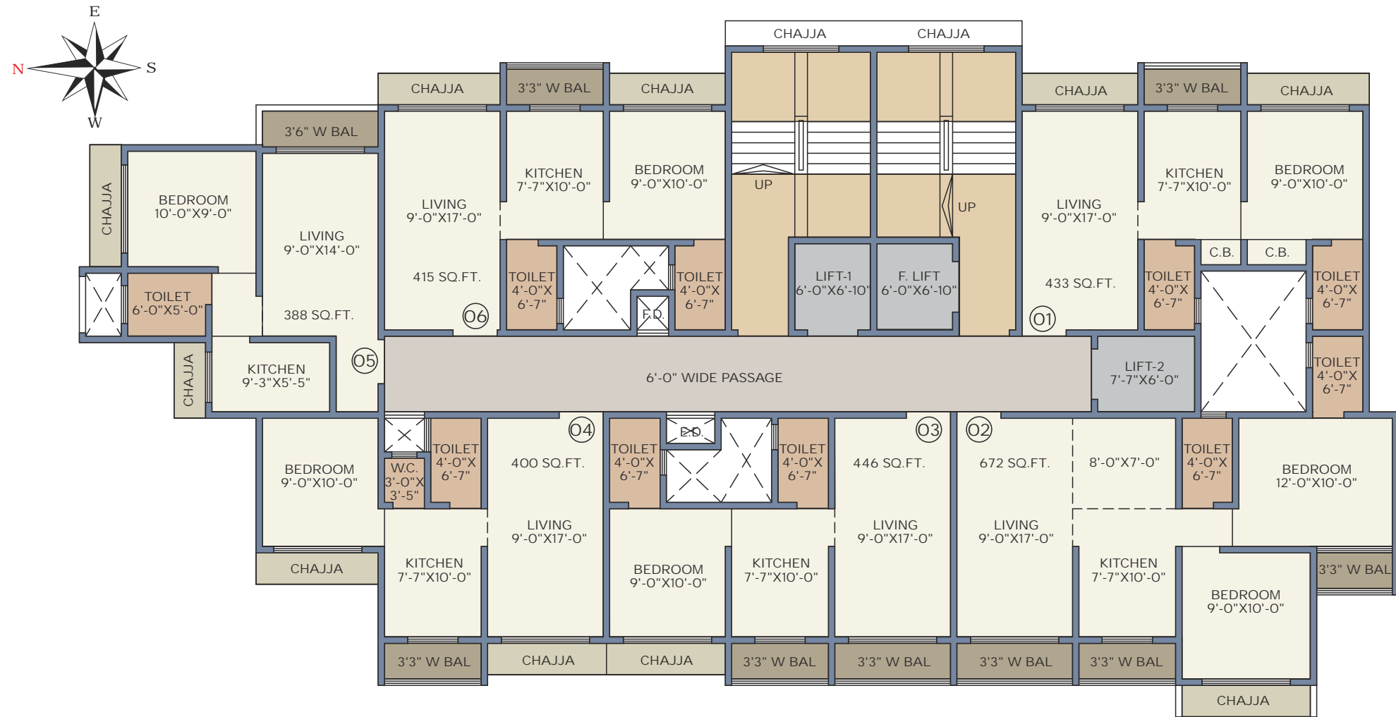
TYPICAL FLOOR PLAN (2ND TO 6TH, 8TH TO 11TH, 13TH TO 16TH, 18TH TO 21ST, 23RD TO 24TH)
